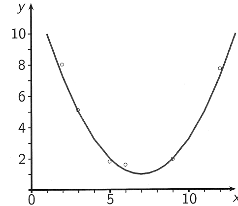
FIGURE 2: Fitting a parabola to data by the method of least squares
