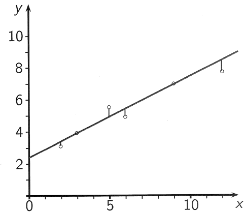
FIGURE 1: Fitting a straight line to data by the method of least squares
