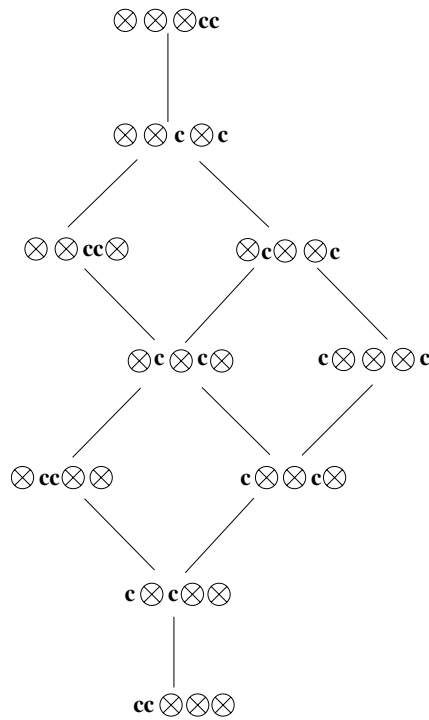
FIGURE 1. The distributive lattice L_{5,2} associated with 2 \mathbf{c} 's and 3 \otimes 's. Observe that the three squares in the lattice correspond to the monomials \mathbf{d}\mathbf{d}\otimes , \mathbf{d}\otimes\mathbf{d} and \otimes\mathbf{d}\mathbf{d} .
