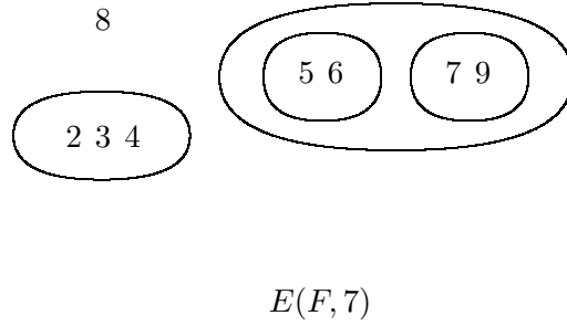
Figure 4: The map E(F, 7) where F = \{\{2, 3, 4\}, \{5, 6\}, \{5, 6, 7\}\} in \Delta_8 .
